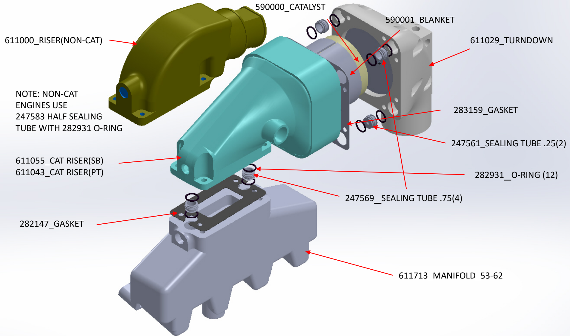
53-62 EXHAUST MANIFOLD PARTS
